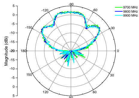
H-plane Co-polarization Pattern
